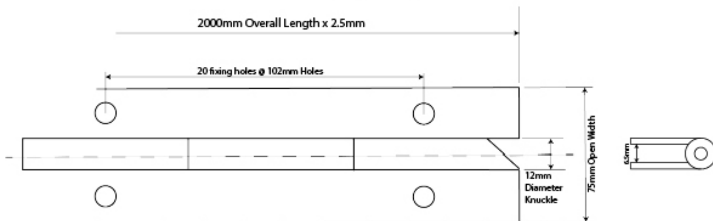
Eclipse Ultra Anti Ligature Continuous Hinge Grade 304 Satin Stainless Steel 200kg Max Weight
